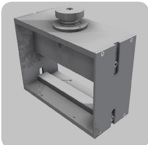
SPLITTING TENSILE APPARATUS FOR CYLINDERS (B-003/ST-010)
